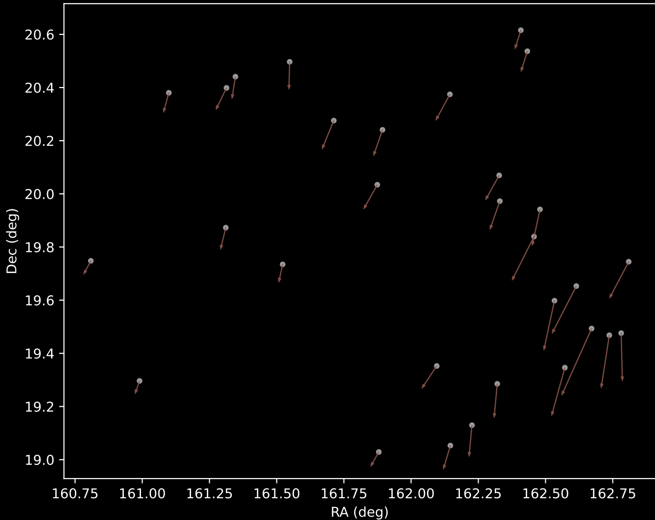
GALAH DR4 Cluster 10 Proper Motion Vectors (n=30)
