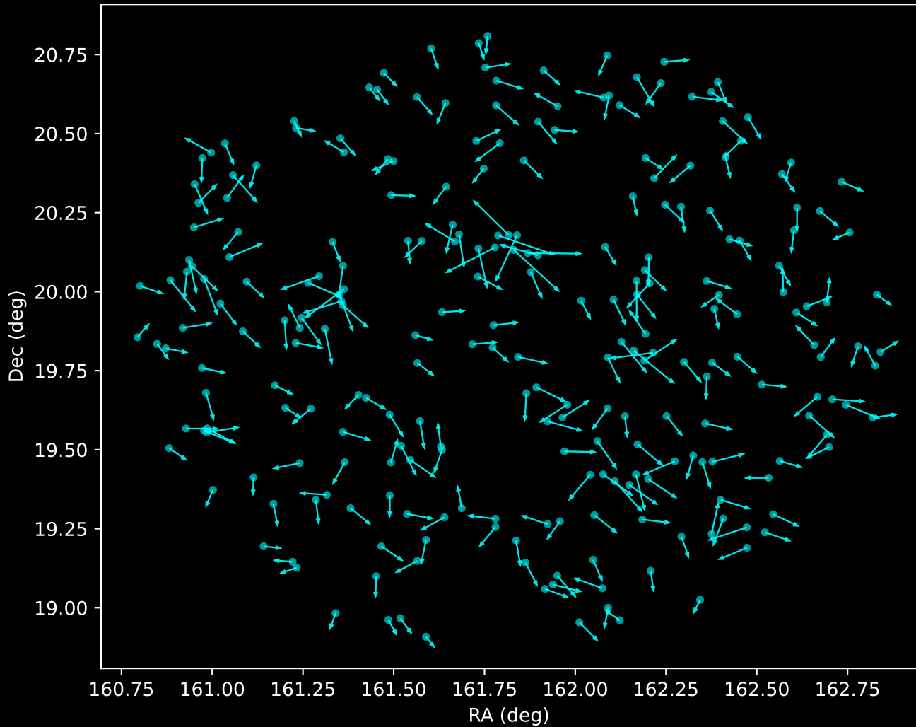
GALAH DR4 Noise Stream Proper Motion Vectors (n=250)
