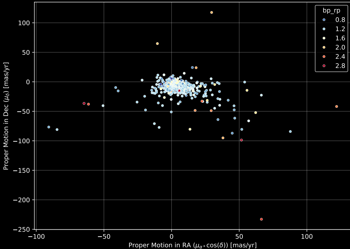
GALAH DR4 Field: [6587] Proper Motion Diagram (n= 471)
