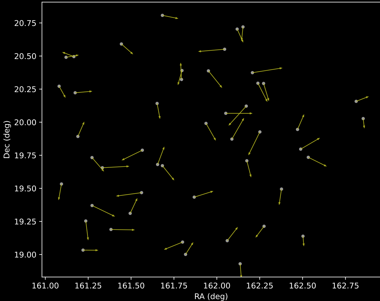
GALAH DR4 Cluster 16 Proper Motion Vectors (n=48)
