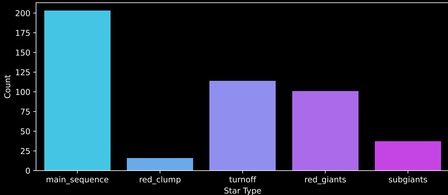
GALAH DR4 Field: [6587] Count plot of Star Type
