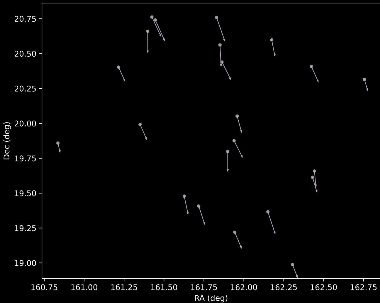
GALAH DR4 Cluster 9 Proper Motion Vectors (n=22)
