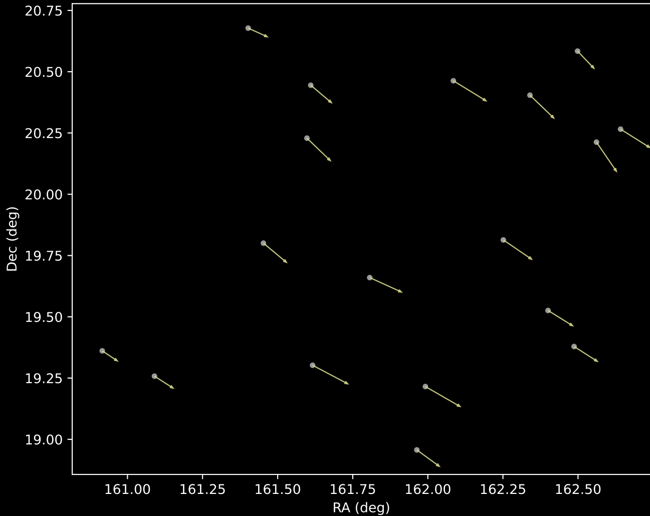
GALAH DR4 Cluster 17 Proper Motion Vectors (n=18)
