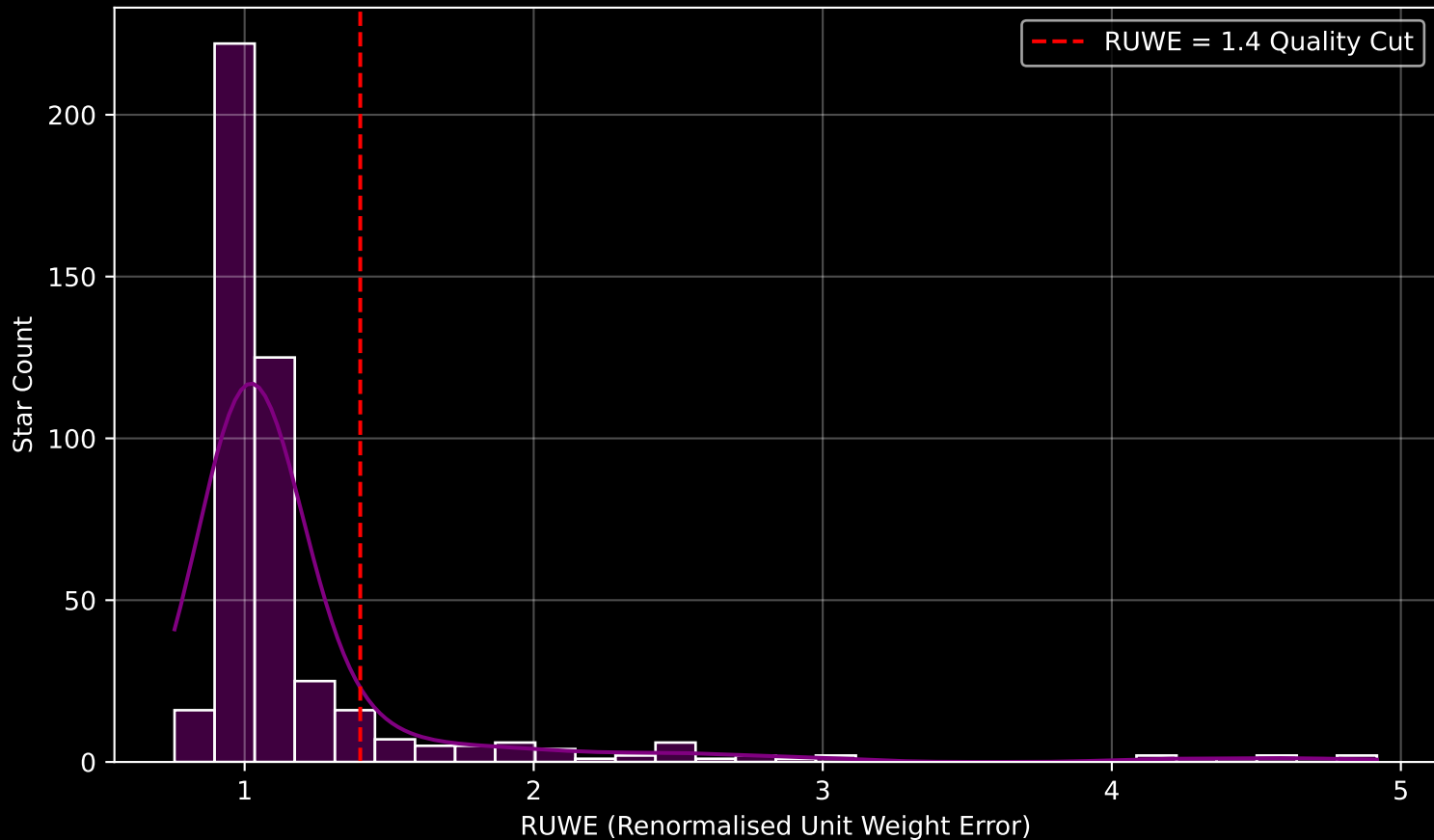
GALAH DR4 Field [6587] RUWE Distribution (n= 454)
